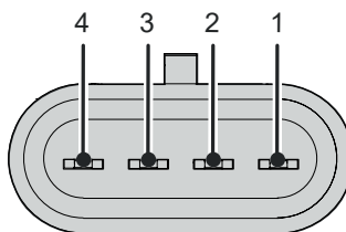
SUPERSEAL™ TE 4-POLE CONNECTOR
