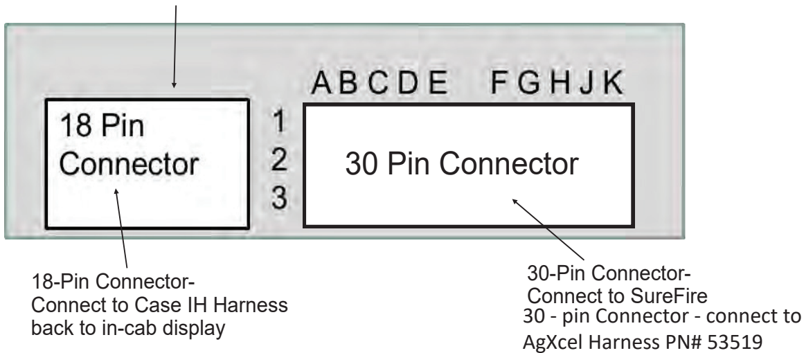
AccuControl Rate and Section Control Module
